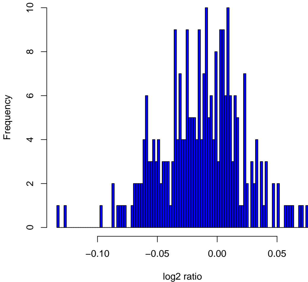
Histogram of log2ratios in 270 HapMap samples at clone Chr4tp-4F3
