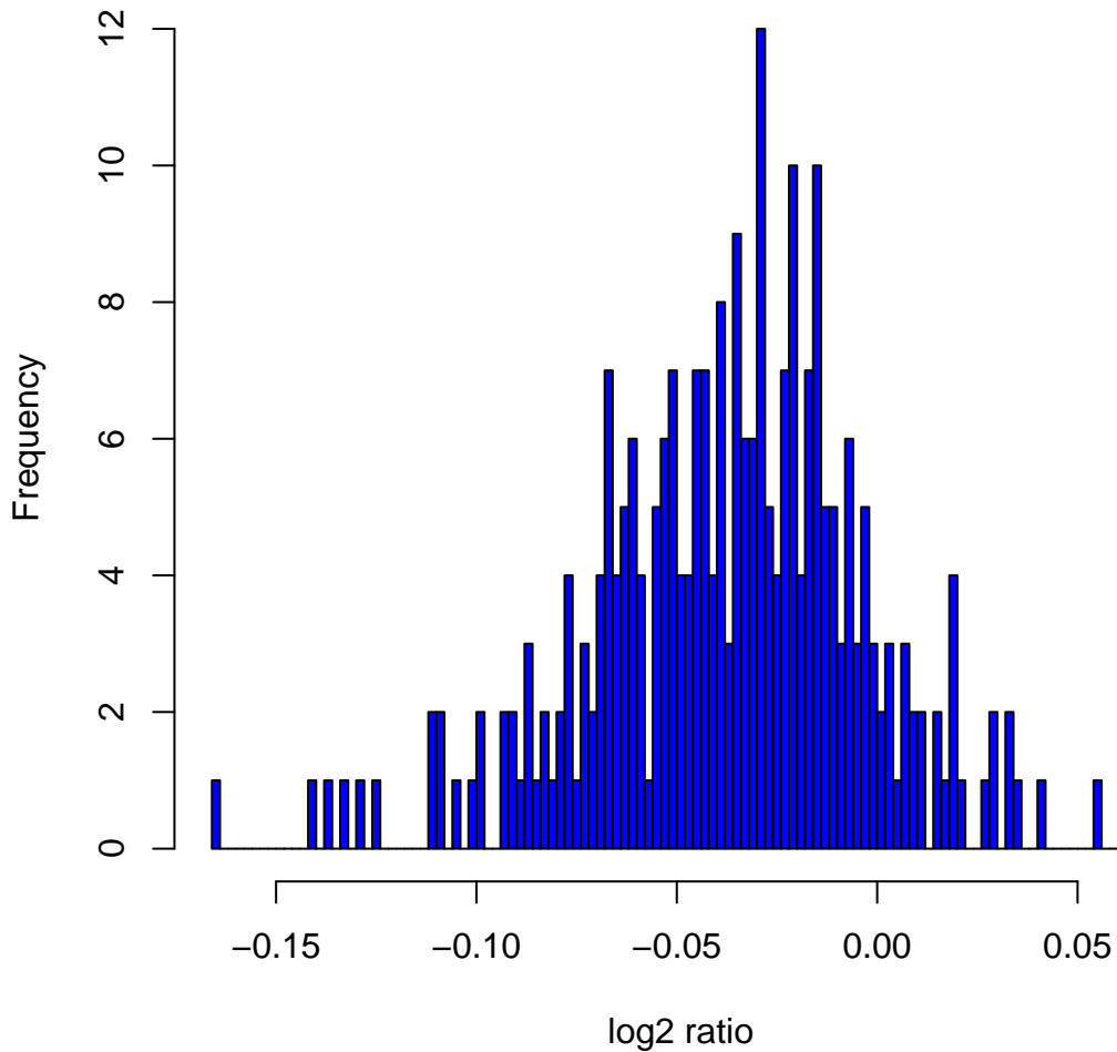
Histogram of log 2 ratios in 270 HapMap samples at clone Chr4tp-4F4
