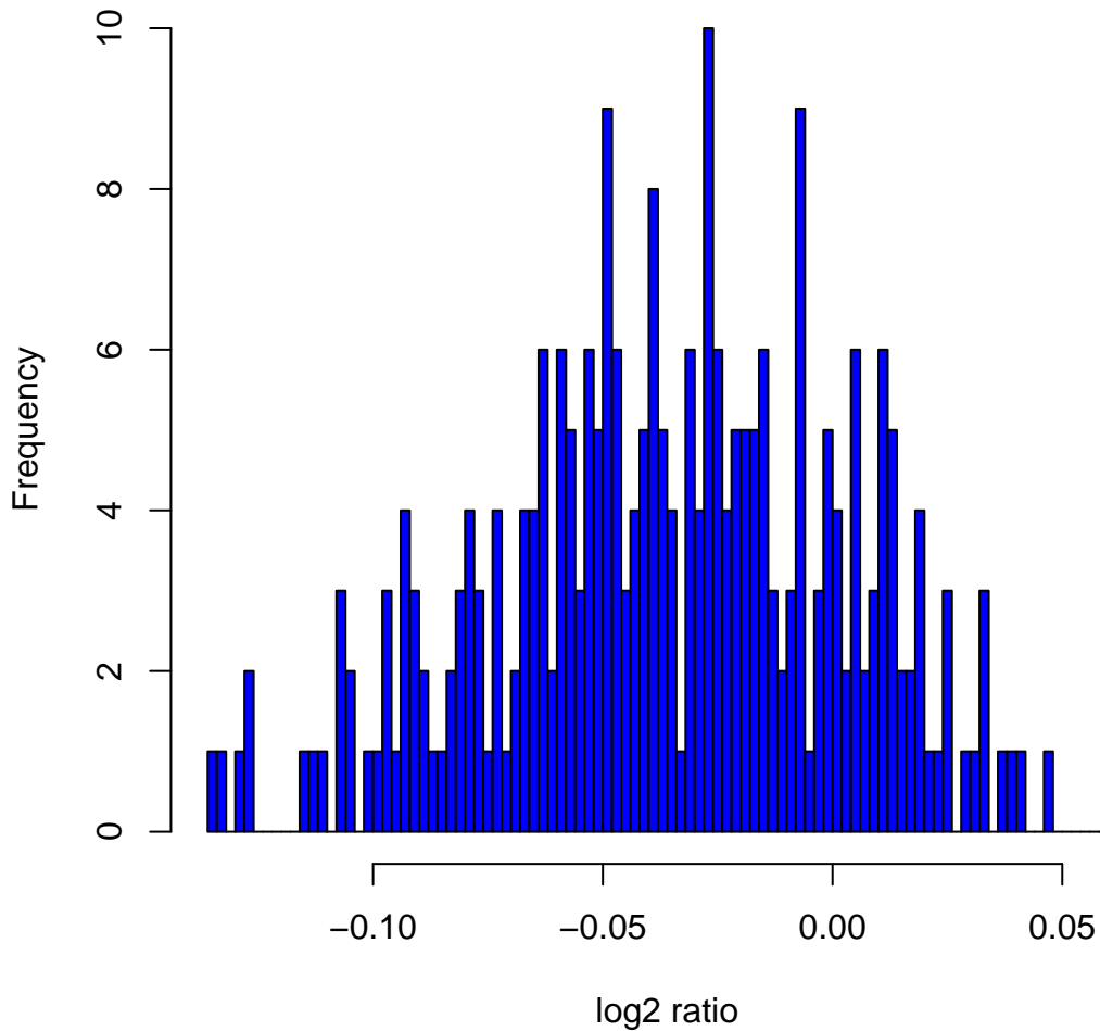
Histogram of \log_2 ratios in 270 HapMap samples at clone Chr4tp-4G12
