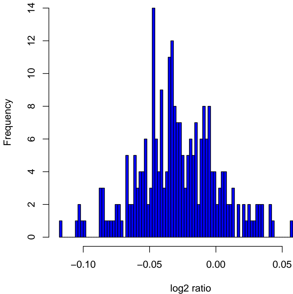
Histogram of log 2 ratios in 270 HapMap samples at clone Chr4tp-4G3
