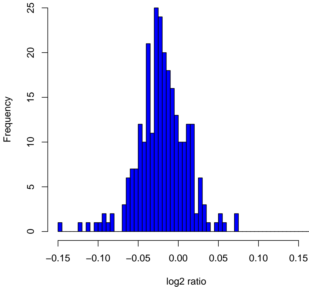
Histogram of \log_2 ratios in 270 HapMap samples at clone Chr4tp-4G4
