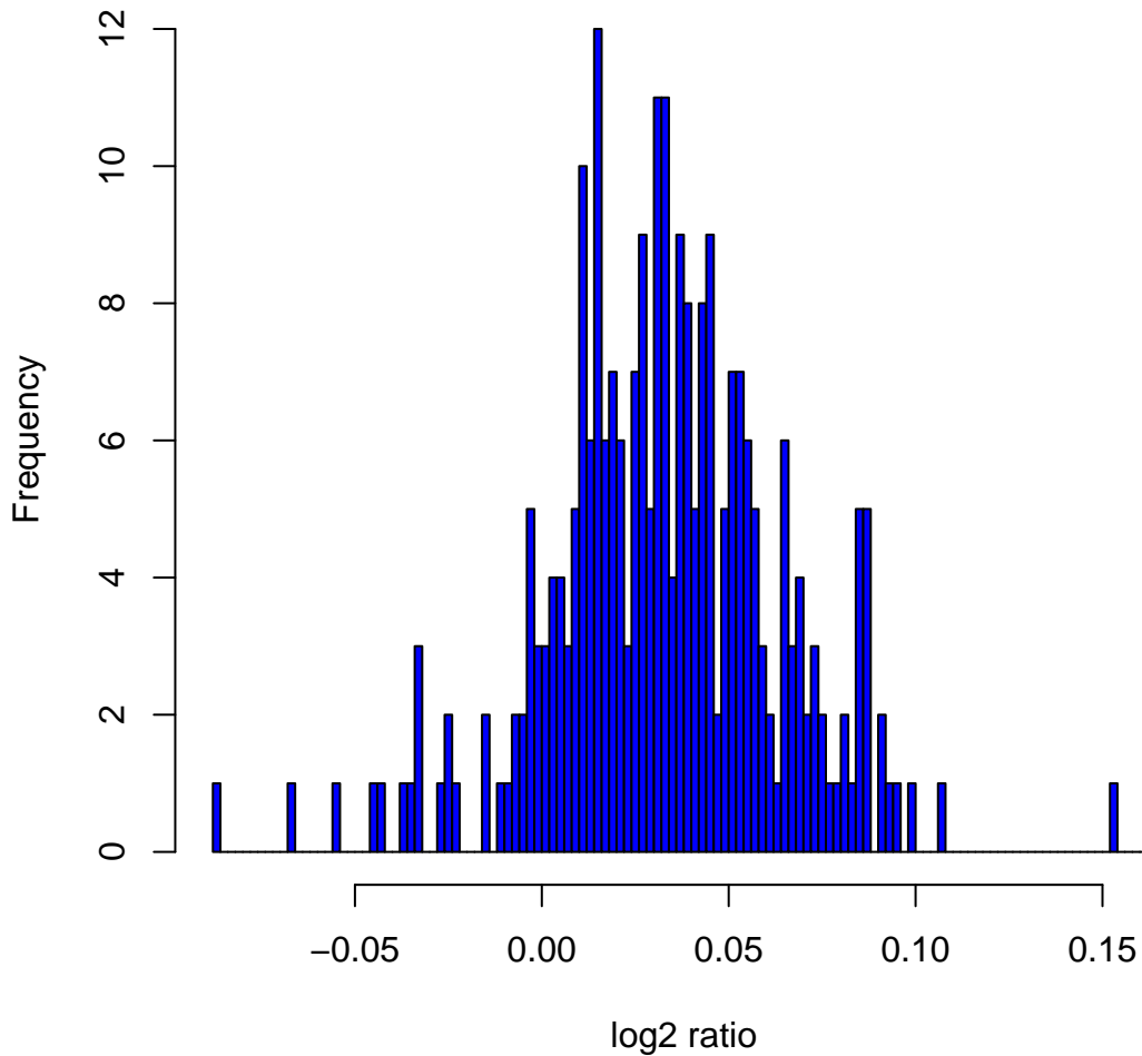
Histogram of log 2 ratios in 270 HapMap samples at clone Chr4tp-4H12
