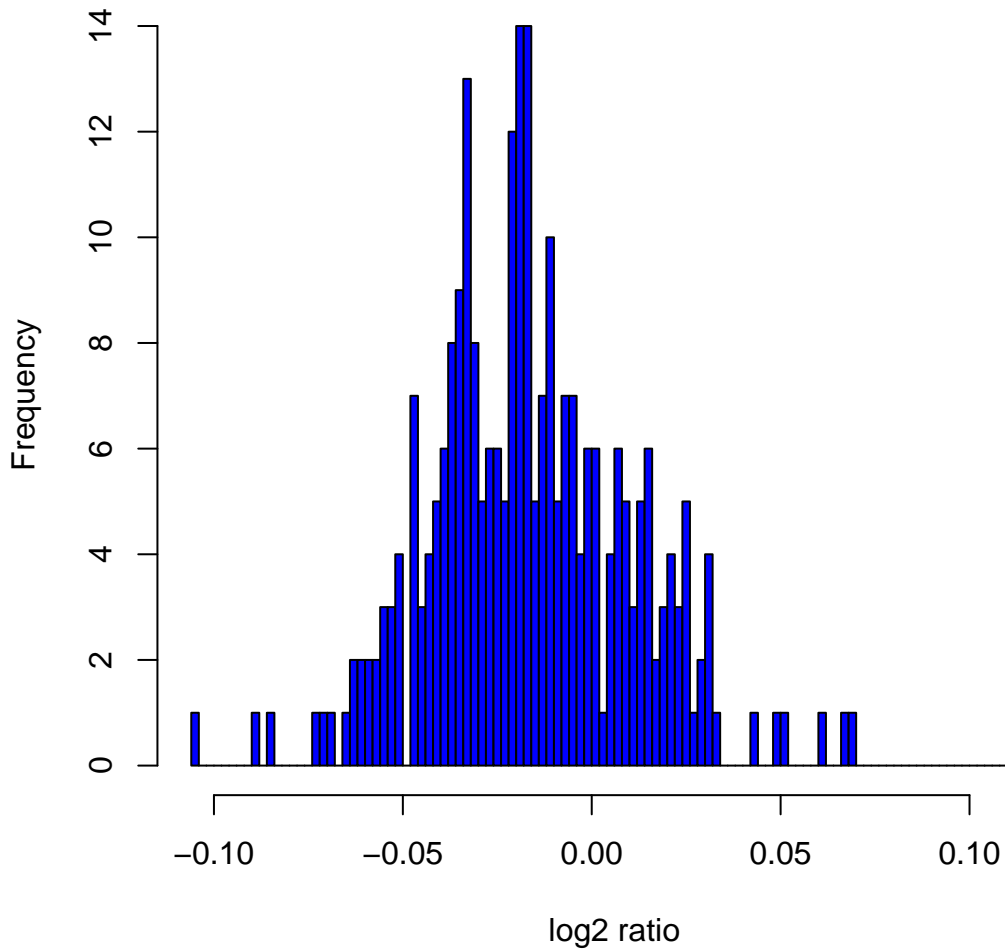
Histogram of log 2 ratios in 270 HapMap samples at clone Chr4tp-4H4
