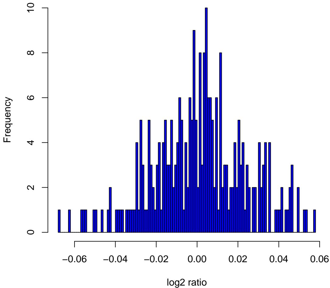
Histogram of \log_2 ratios in 270 HapMap samples at clone Chr4tp-4H5
