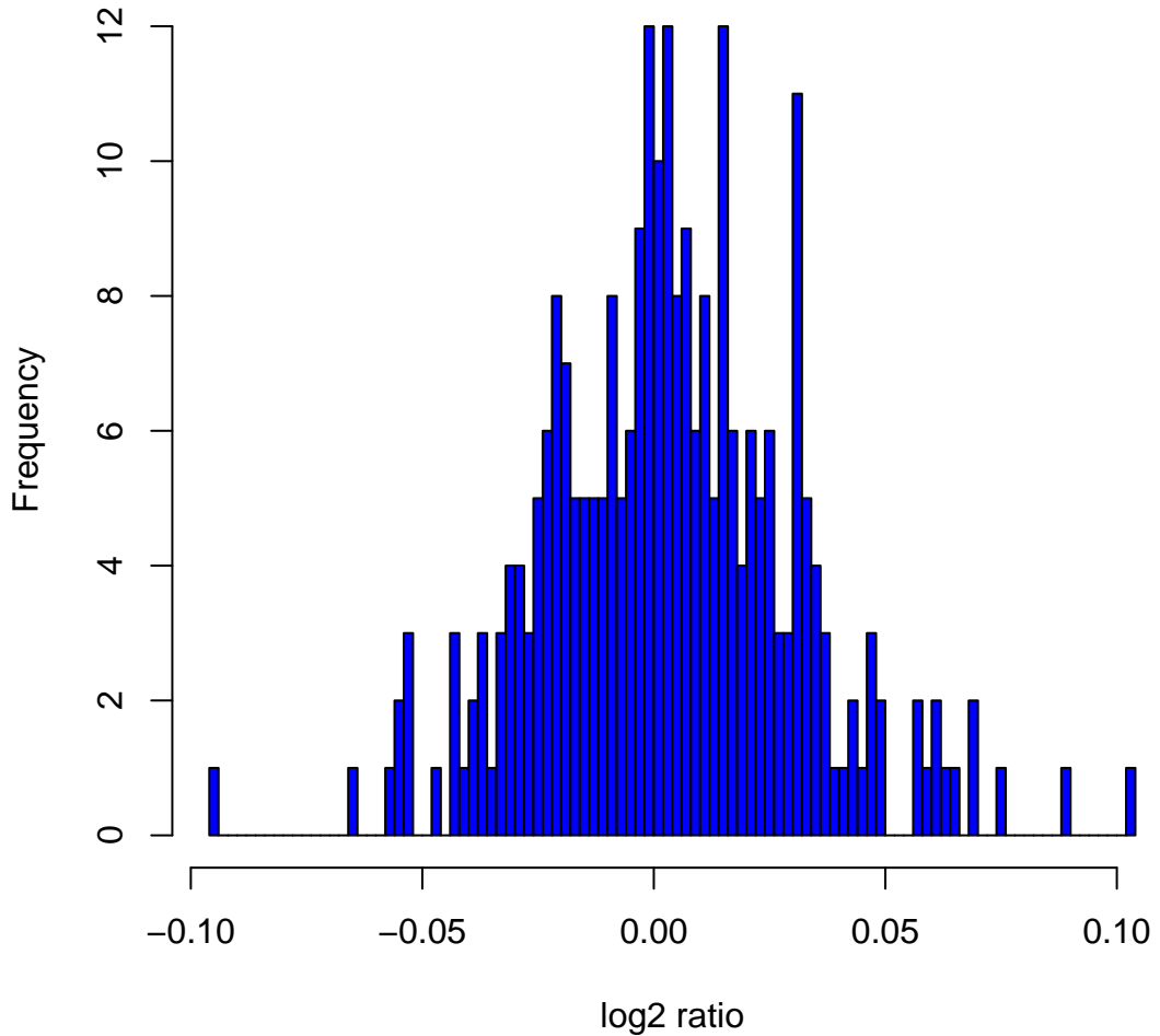
Histogram of \log_2 ratios in 270 HapMap samples at clone Chr4tp-5B12
