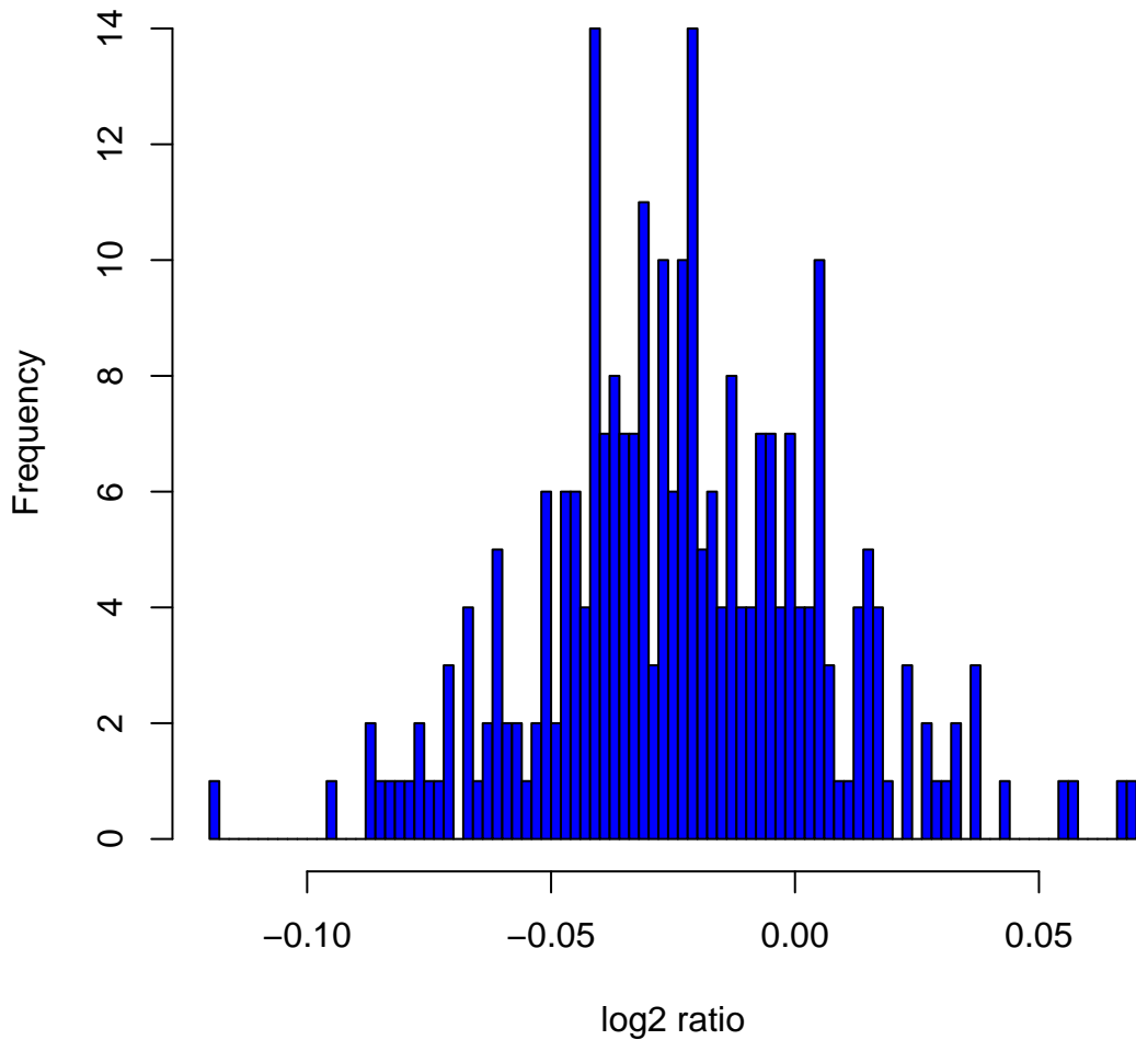
Histogram of log 2 ratios in 270 HapMap samples at clone Chr4tp-5B3
