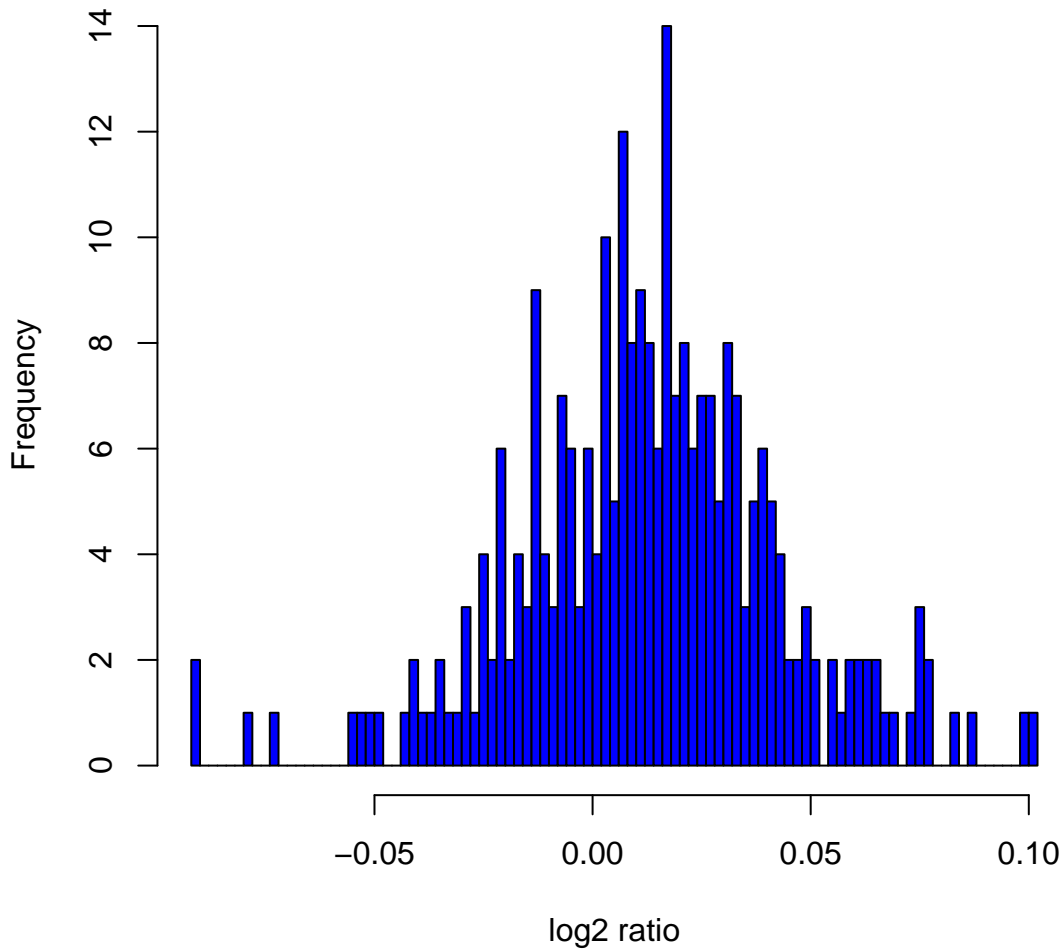
Histogram of log 2 ratios in 270 HapMap samples at clone Chr4tp-5B5
