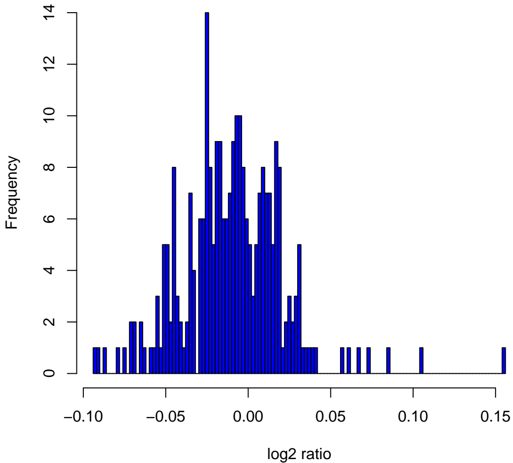
Histogram of log 2 ratios in 270 HapMap samples at clone Chr4tp-5C3
