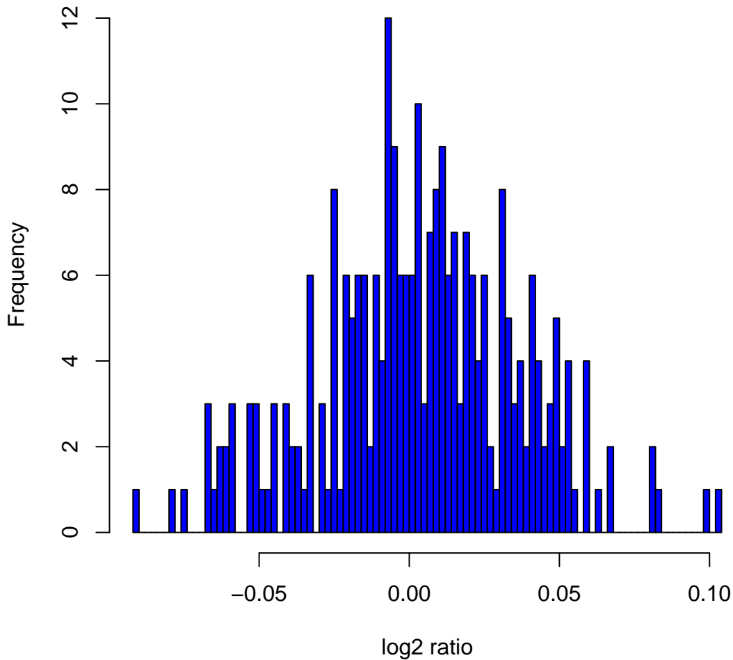
Histogram of log 2 ratios in 270 HapMap samples at clone Chr4tp-5C6
