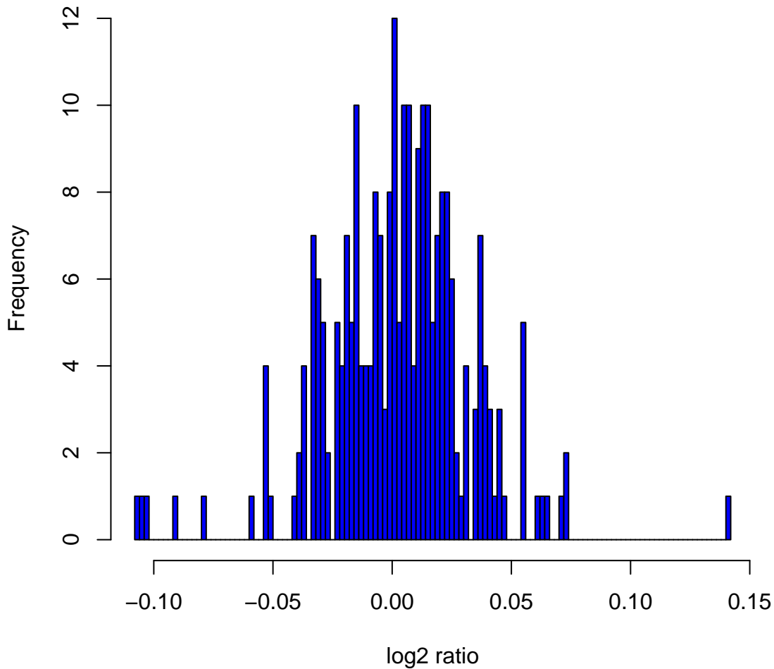
Histogram of \log_2 ratios in 270 HapMap samples at clone Chr4tp-5D1
