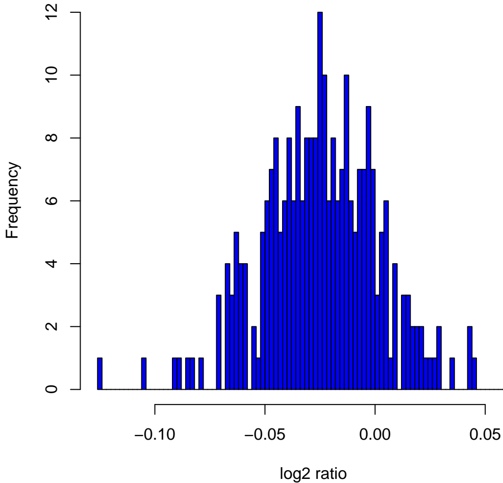
Histogram of log 2 ratios in 270 HapMap samples at clone Chr4tp-5D2
