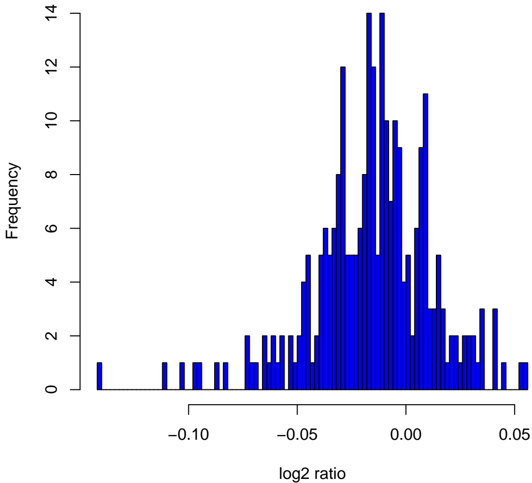
Histogram of log 2 ratios in 270 HapMap samples at clone Chr4tp-5D9
