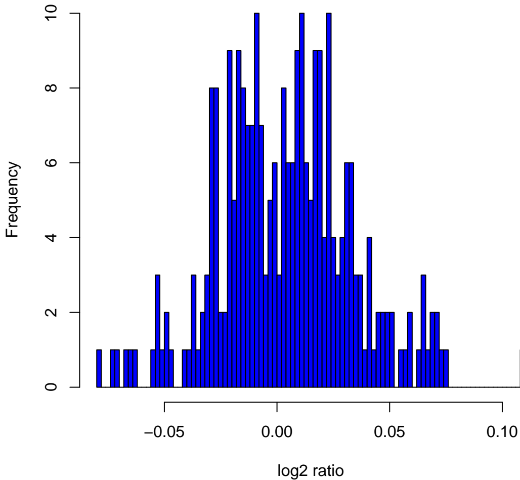
Histogram of \log_2 ratios in 270 HapMap samples at clone Chr4tp-5E11
