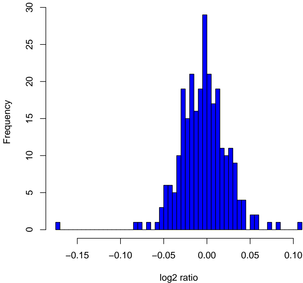
Histogram of log 2 ratios in 270 HapMap samples at clone Chr4tp-5E12
