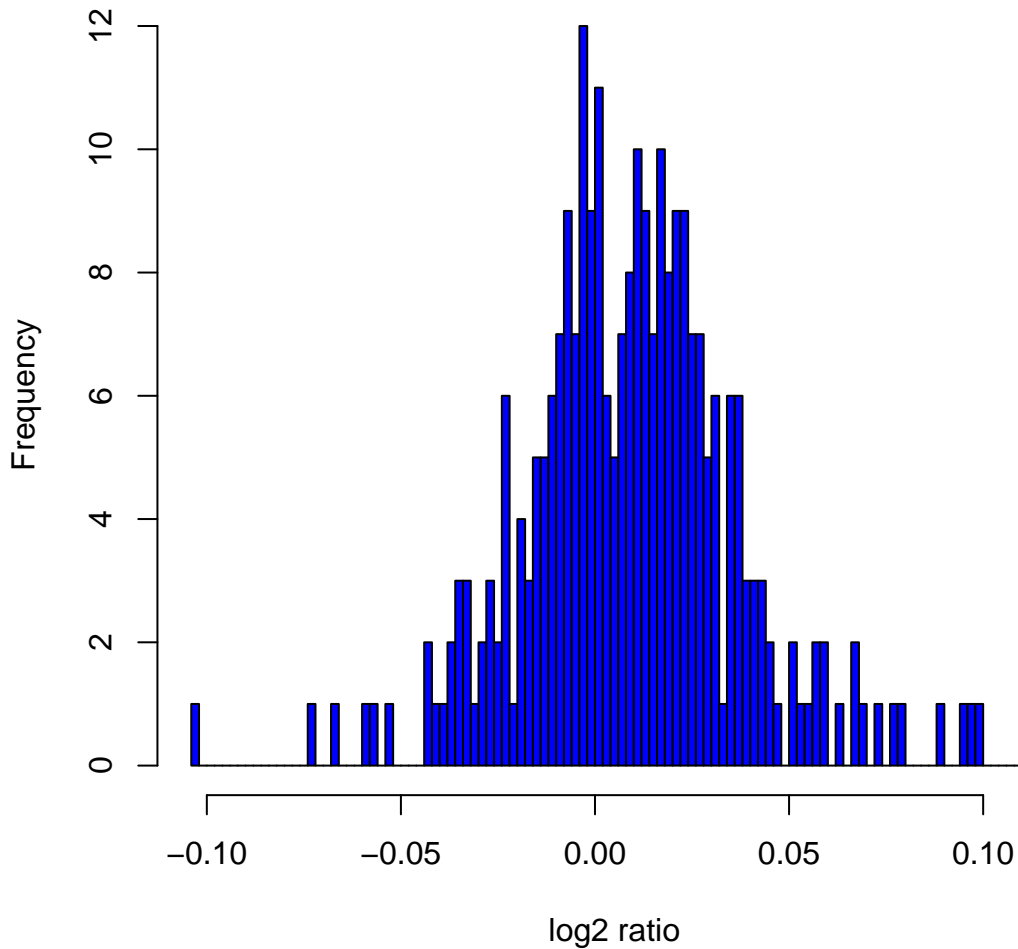
Histogram of log 2 ratios in 270 HapMap samples at clone Chr4tp-5E7
