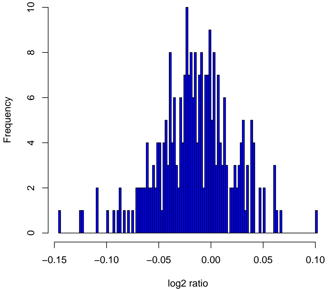
Histogram of log2ratios in 270 HapMap samples at clone Chr4tp-5F2
