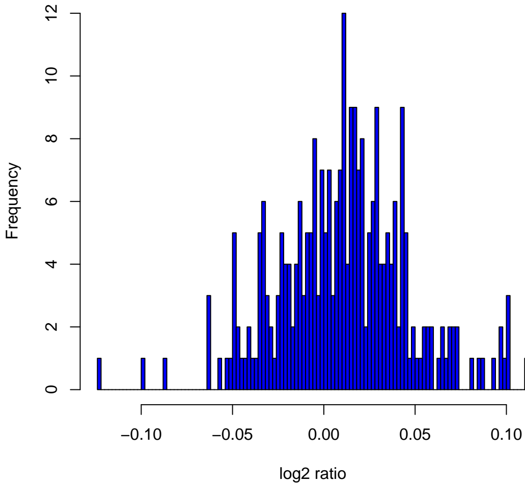
Histogram of log 2 ratios in 270 HapMap samples at clone Chr4tp-5G1
