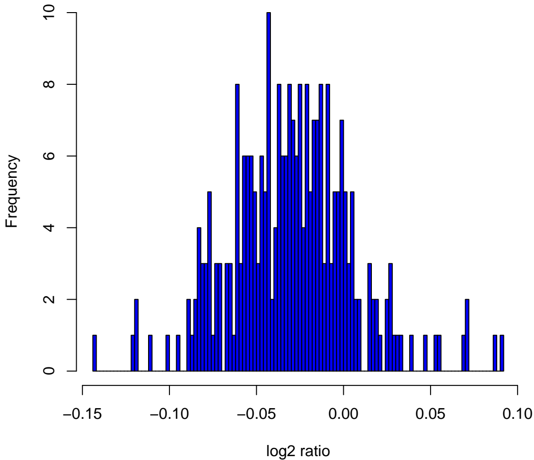
Histogram of log2ratios in 270 HapMap samples at clone Chr4tp-5G3
