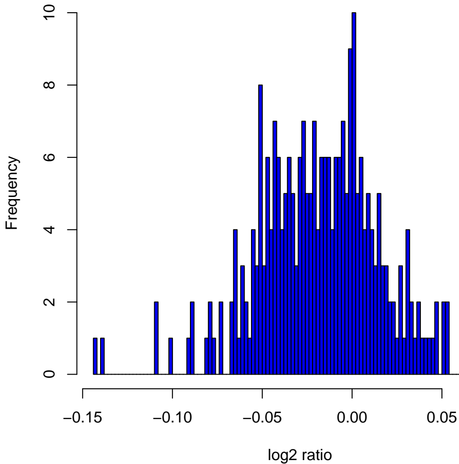
Histogram of \log_2 ratios in 270 HapMap samples at clone Chr4tp-5H6
