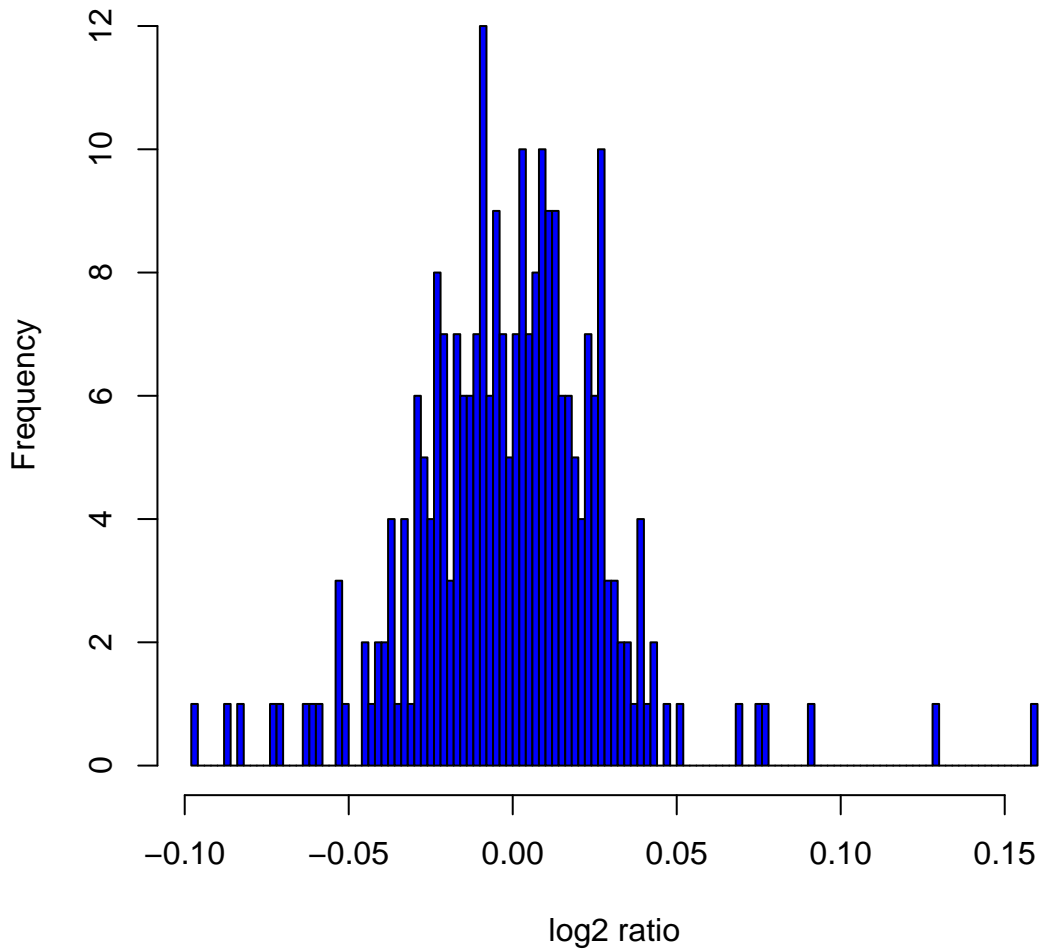
Histogram of log 2 ratios in 270 HapMap samples at clone Chr4tp-5H9
