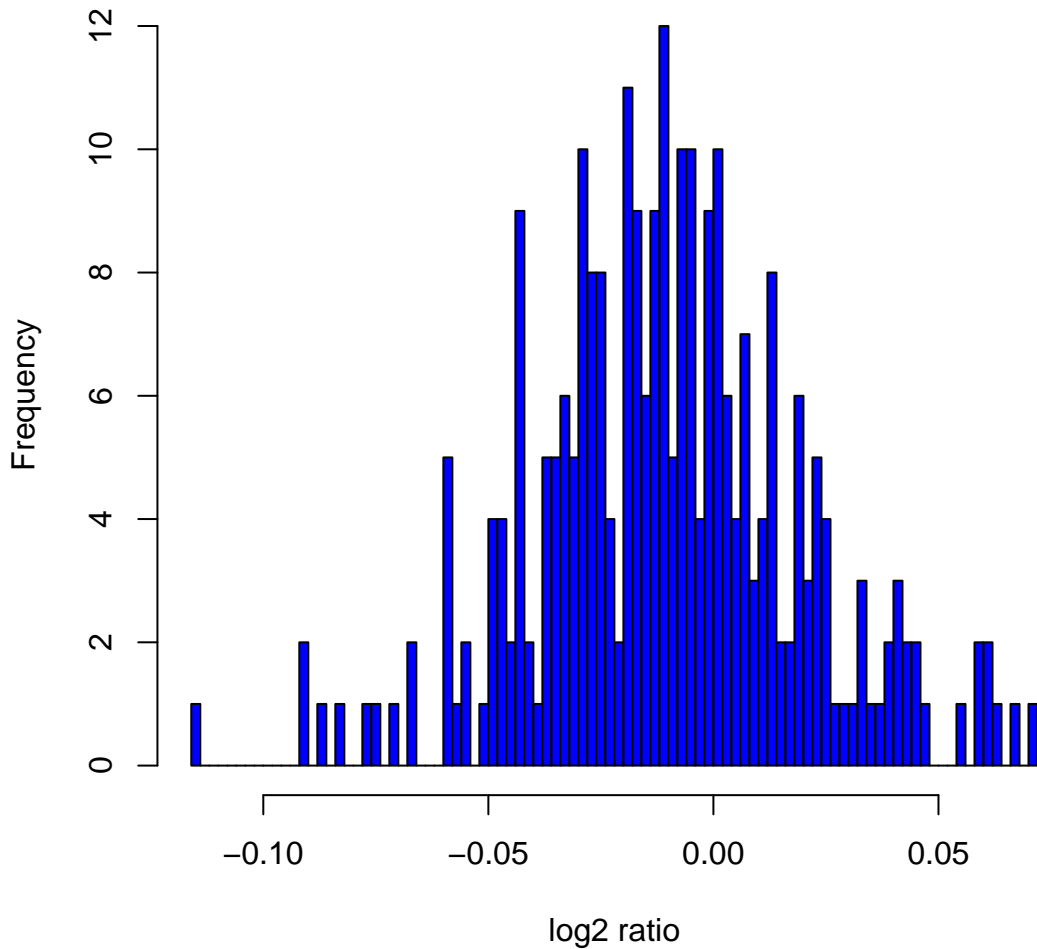
Histogram of \log_2 ratios in 270 HapMap samples at clone Chr4tp-6A3
