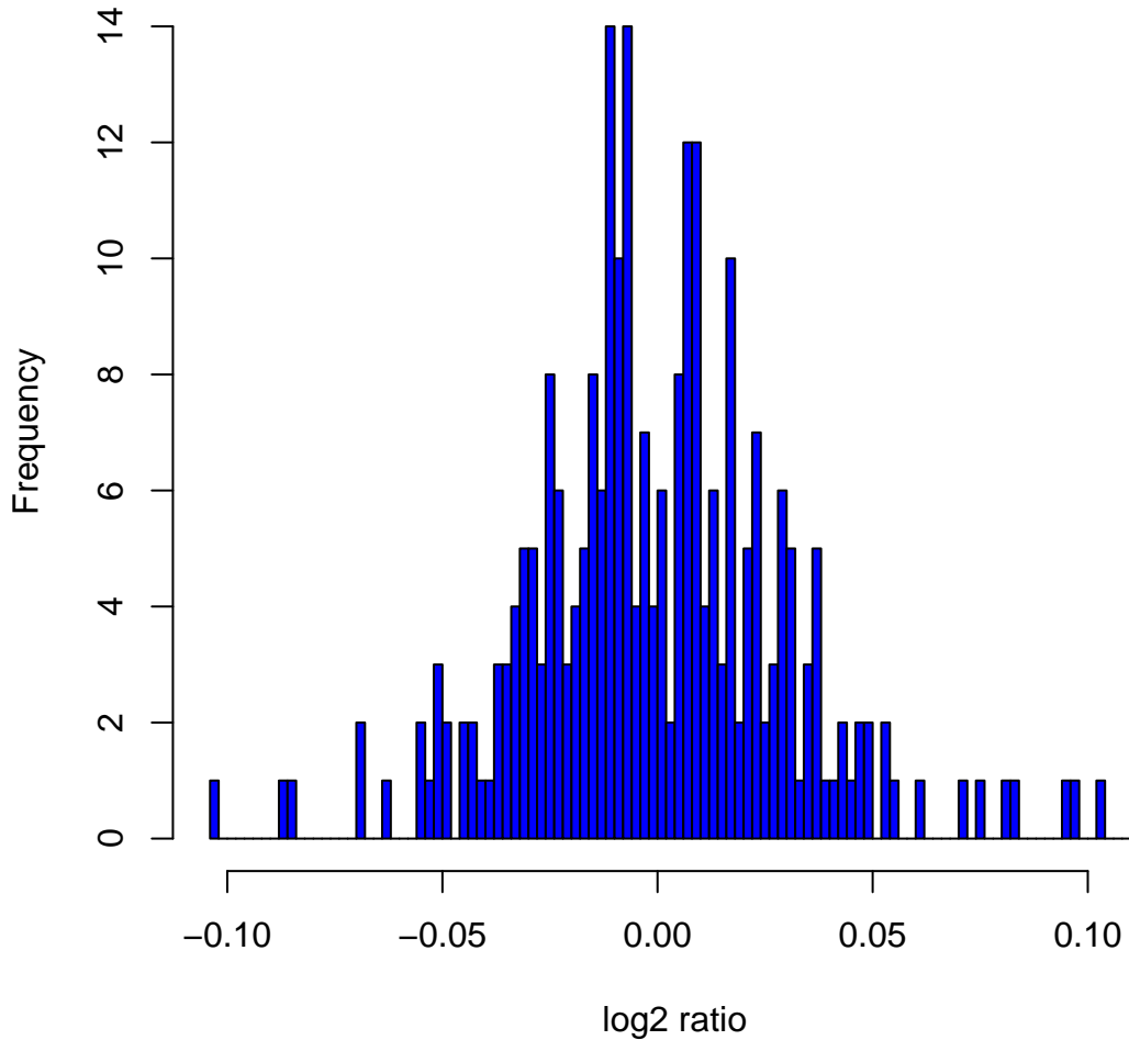
Histogram of log 2 ratios in 270 HapMap samples at clone Chr4tp-6B12
