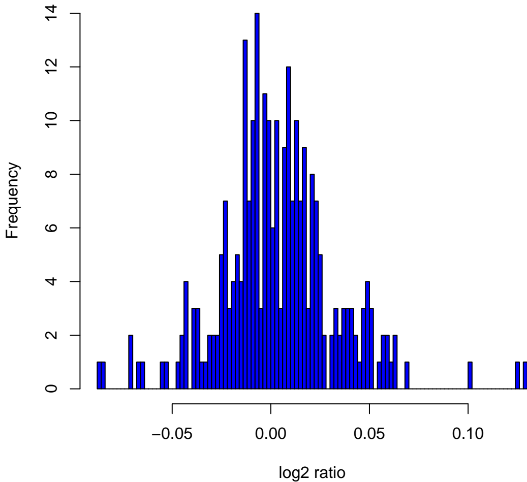
Histogram of log 2 ratios in 270 HapMap samples at clone Chr4tp-6D2
