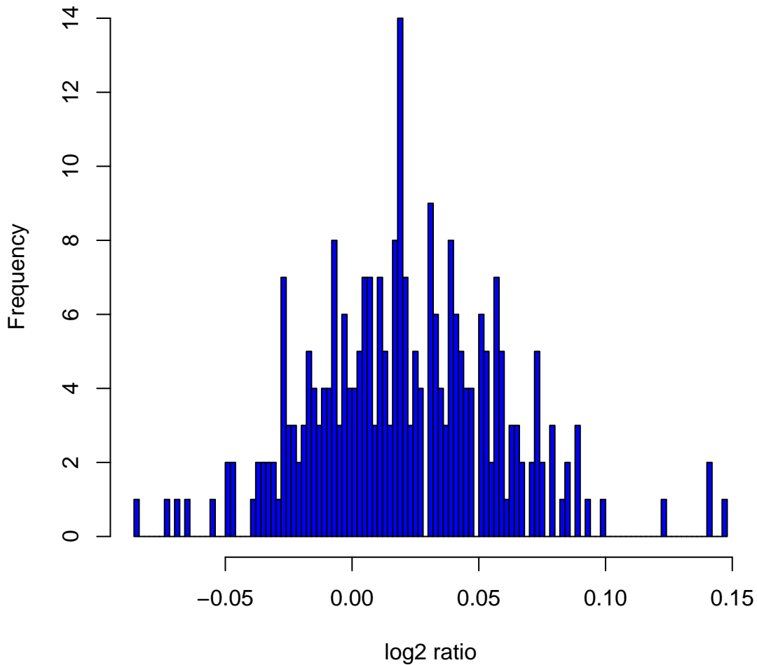
Histogram of log2ratios in 270 HapMap samples at clone Chr4tp-6E1
