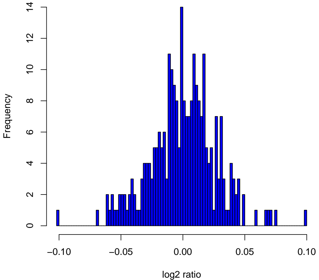
Histogram of log2ratios in 270 HapMap samples at clone Chr4tp-6F5
