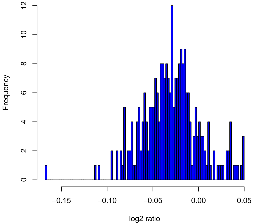
Histogram of log2ratios in 270 HapMap samples at clone Chr4tp-6F9
