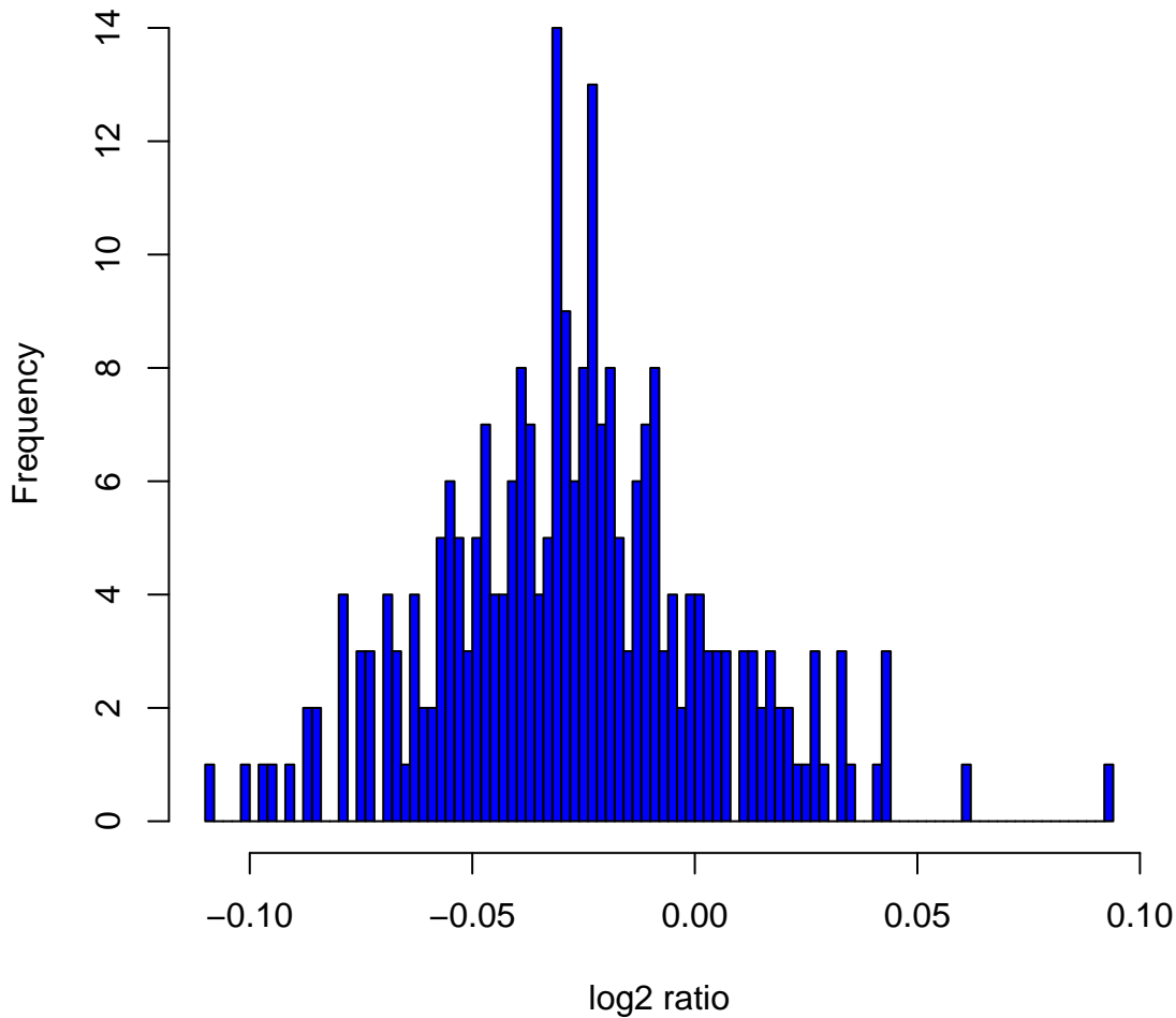
Histogram of log2ratios in 270 HapMap samples at clone Chr4tp-6H7
