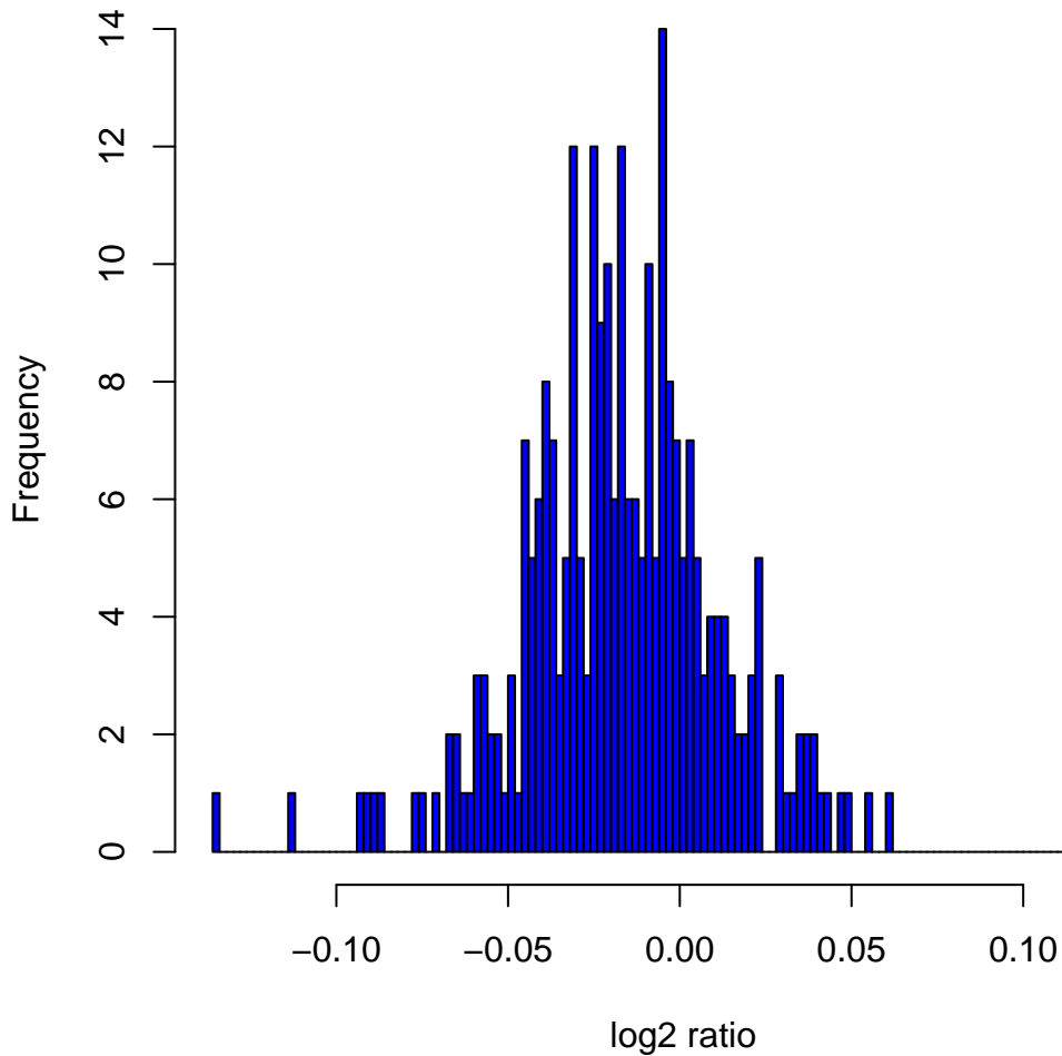
Histogram of \log_2 ratios in 270 HapMap samples at clone Chr4tp-7A10
