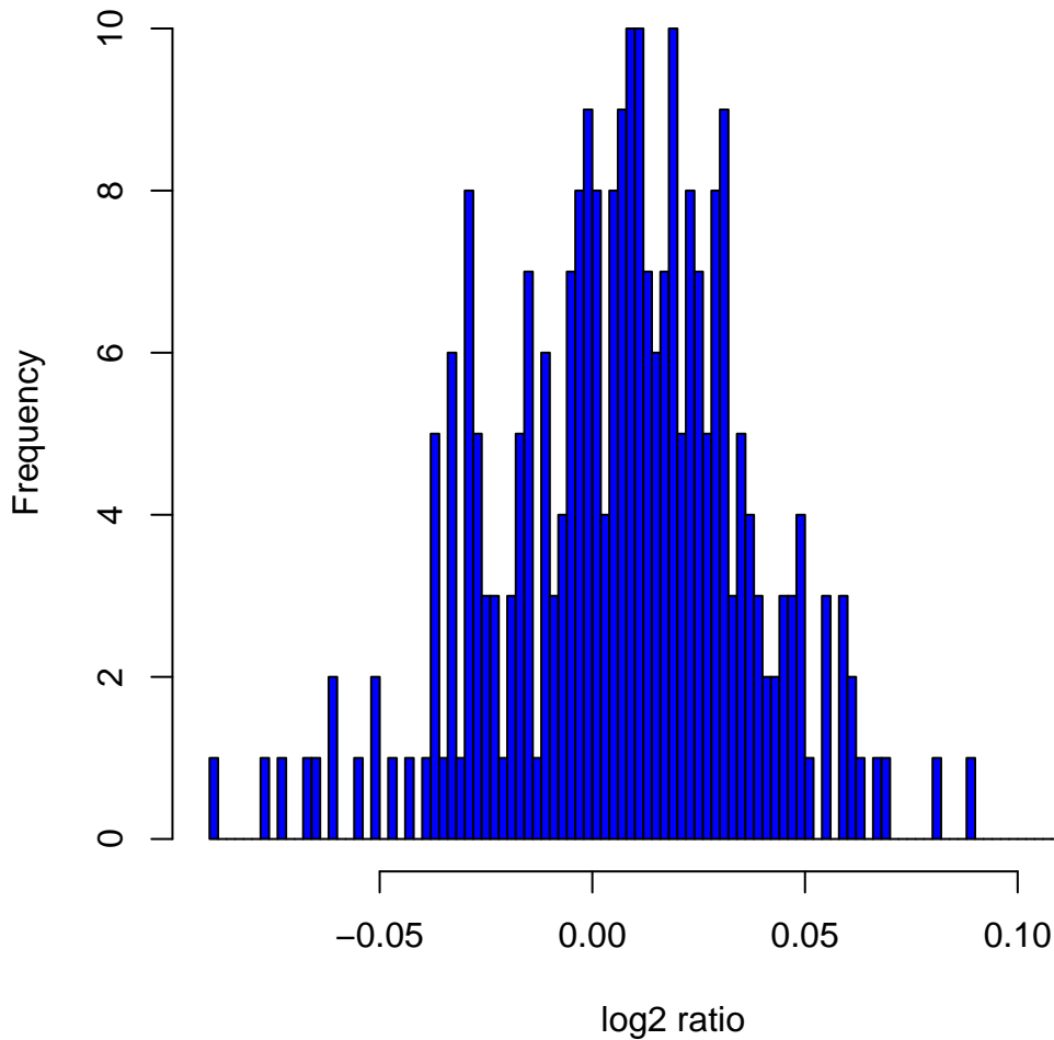
Histogram of \log_2 ratios in 270 HapMap samples at clone Chr4tp-7A12
