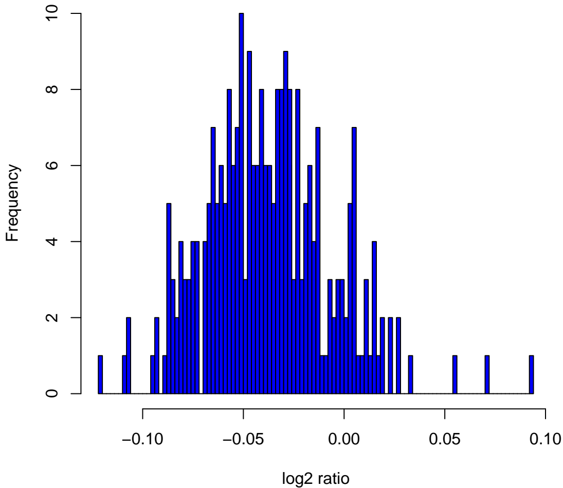
Histogram of log 2 ratios in 270 HapMap samples at clone Chr4tp-7A5
