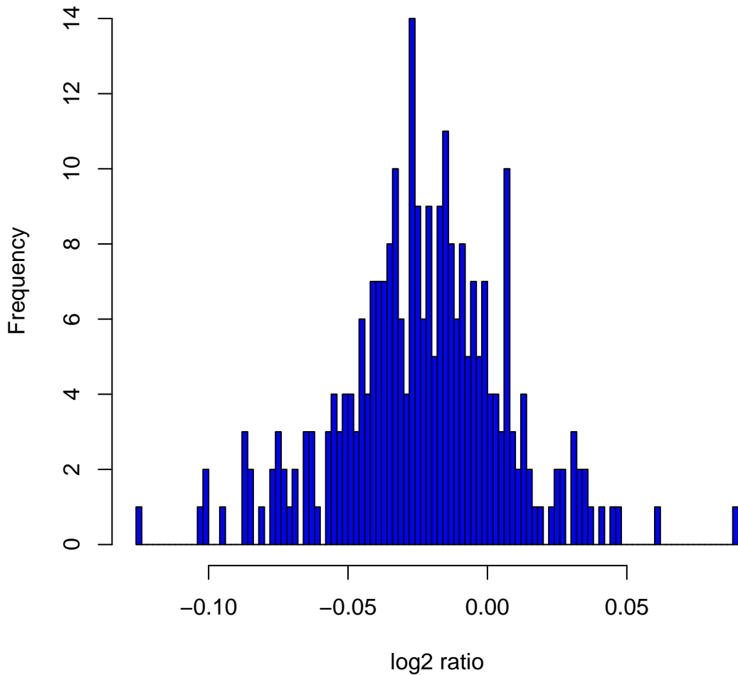
Histogram of \log_2 ratios in 270 HapMap samples at clone Chr4tp-7A9
