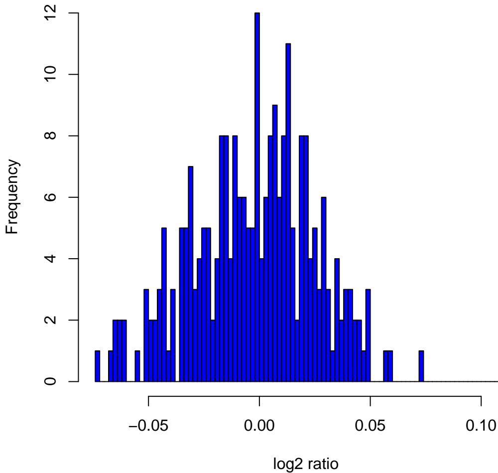
Histogram of log 2 ratios in 270 HapMap samples at clone Chr4tp-7B1
