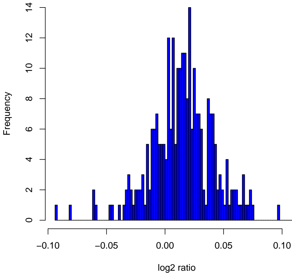
Histogram of \log_2 ratios in 270 HapMap samples at clone Chr4tp-7C2
