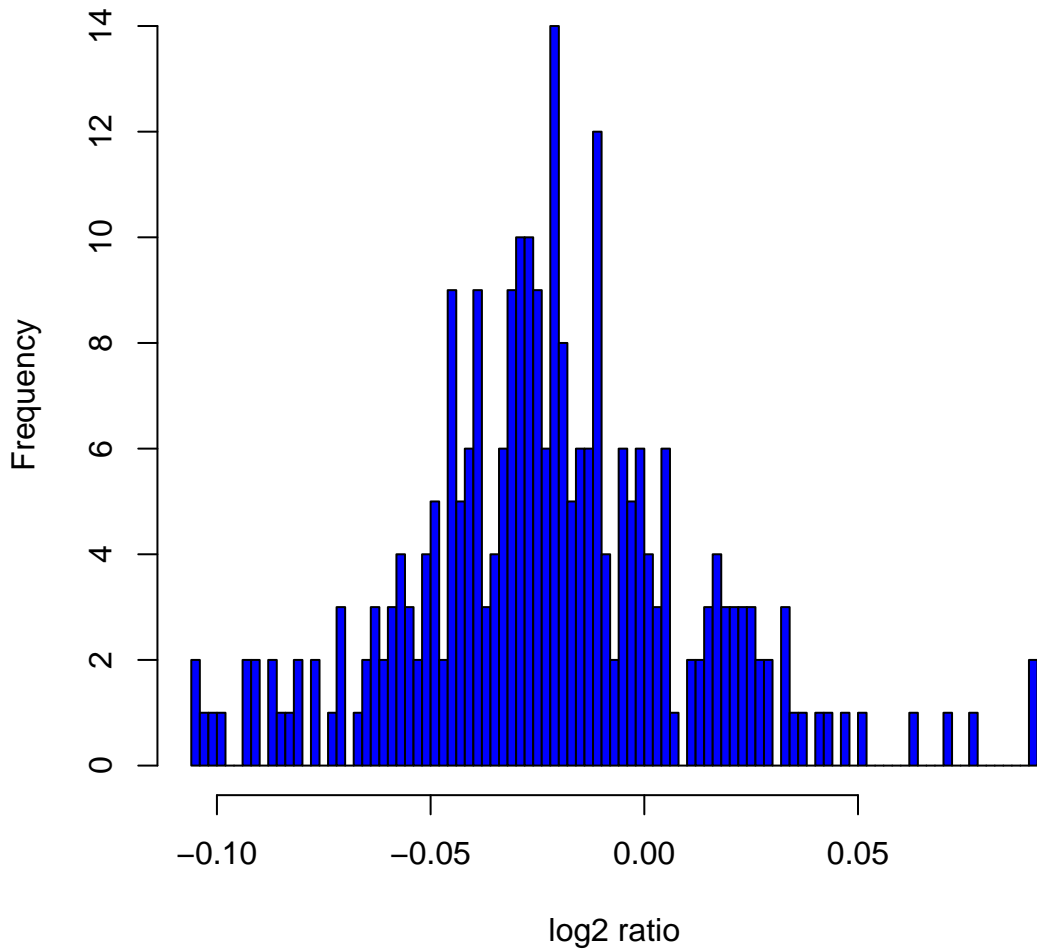
Histogram of log 2 ratios in 270 HapMap samples at clone Chr4tp-7D3
