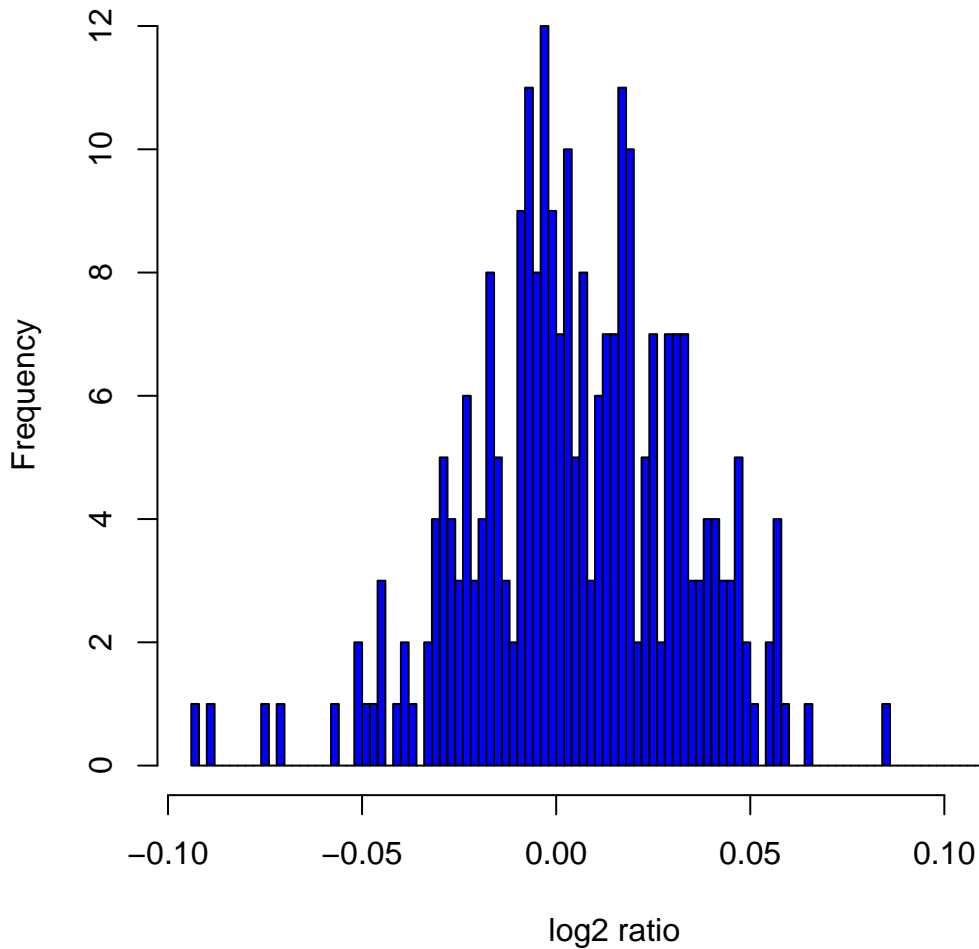
Histogram of \log_2 ratios in 270 HapMap samples at clone Chr4tp-7D4
