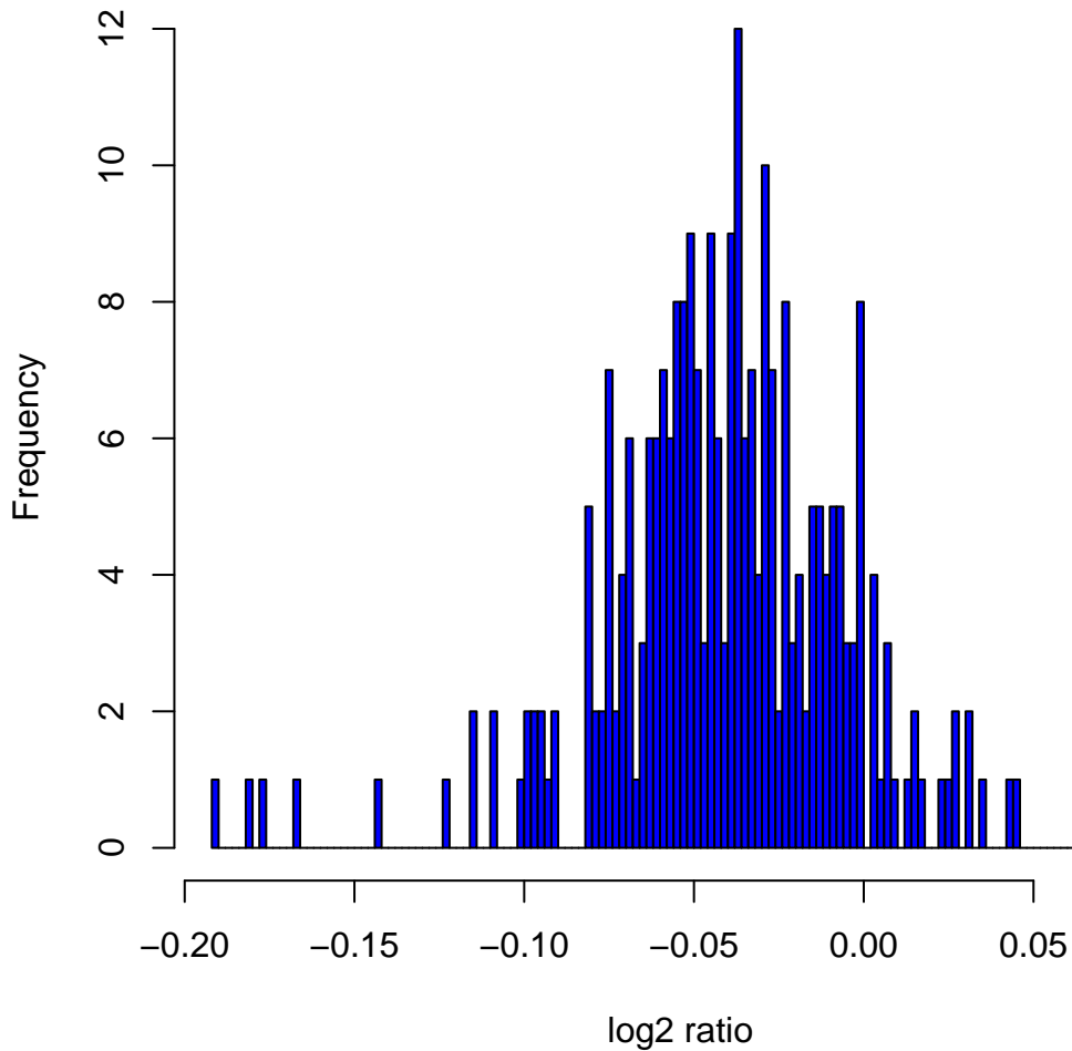
Histogram of log 2 ratios in 270 HapMap samples at clone Chr4tp-7E1
