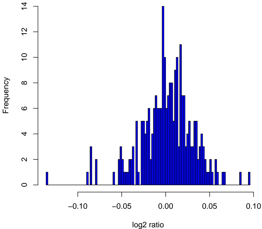
Histogram of log 2 ratios in 270 HapMap samples at clone Chr4tp-7H7
