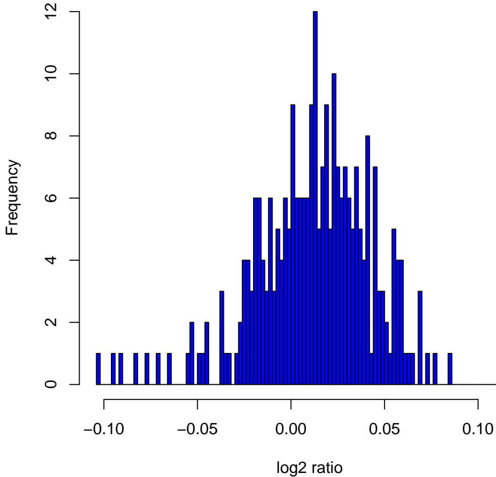
Histogram of log 2 ratios in 270 HapMap samples at clone Chr4tp-8A12
