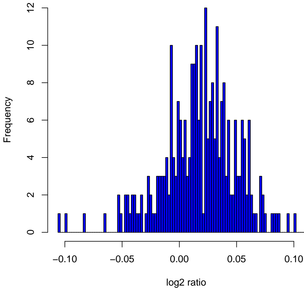
Histogram of \log_2 ratios in 270 HapMap samples at clone Chr4tp-8B4
