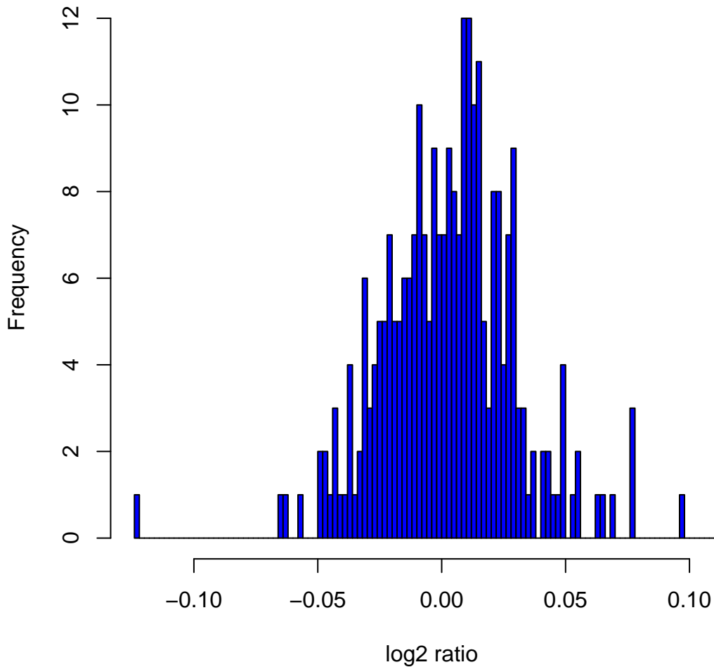
Histogram of \log_2 ratios in 270 HapMap samples at clone Chr4tp-8C3
