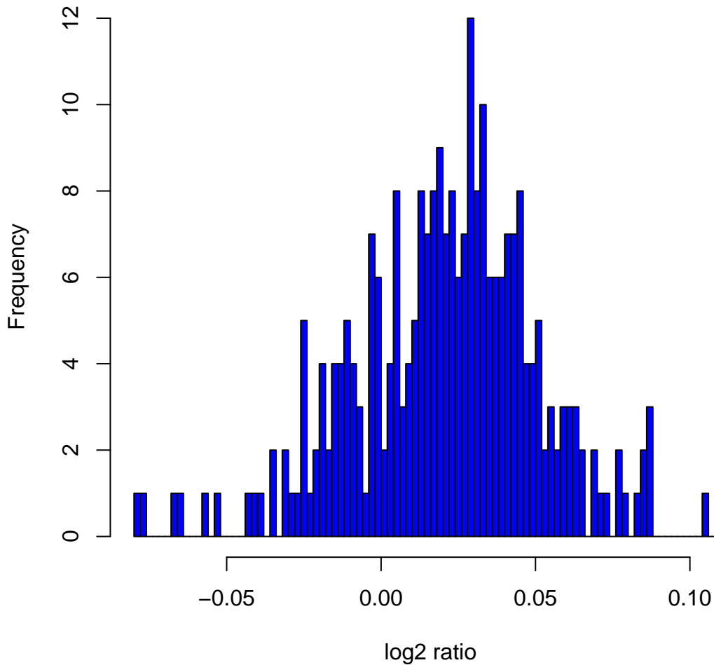
Histogram of log2ratios in 270 HapMap samples at clone Chr4tp-8C6
