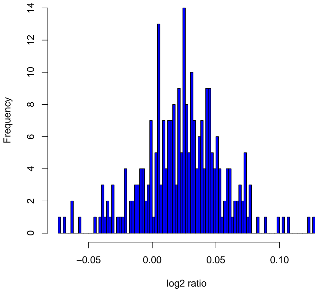
Histogram of log 2 ratios in 270 HapMap samples at clone Chr4tp-8D2
