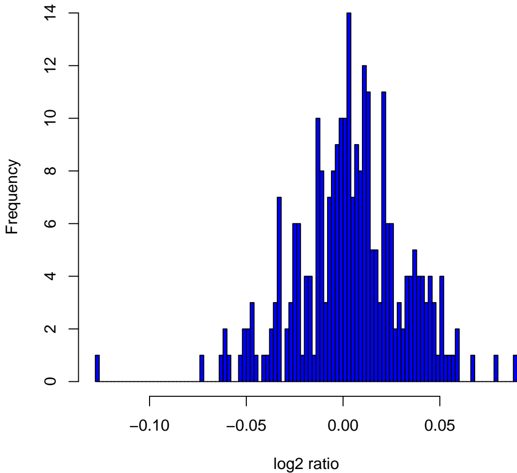
Histogram of log2ratios in 270 HapMap samples at clone Chr4tp-8E11
