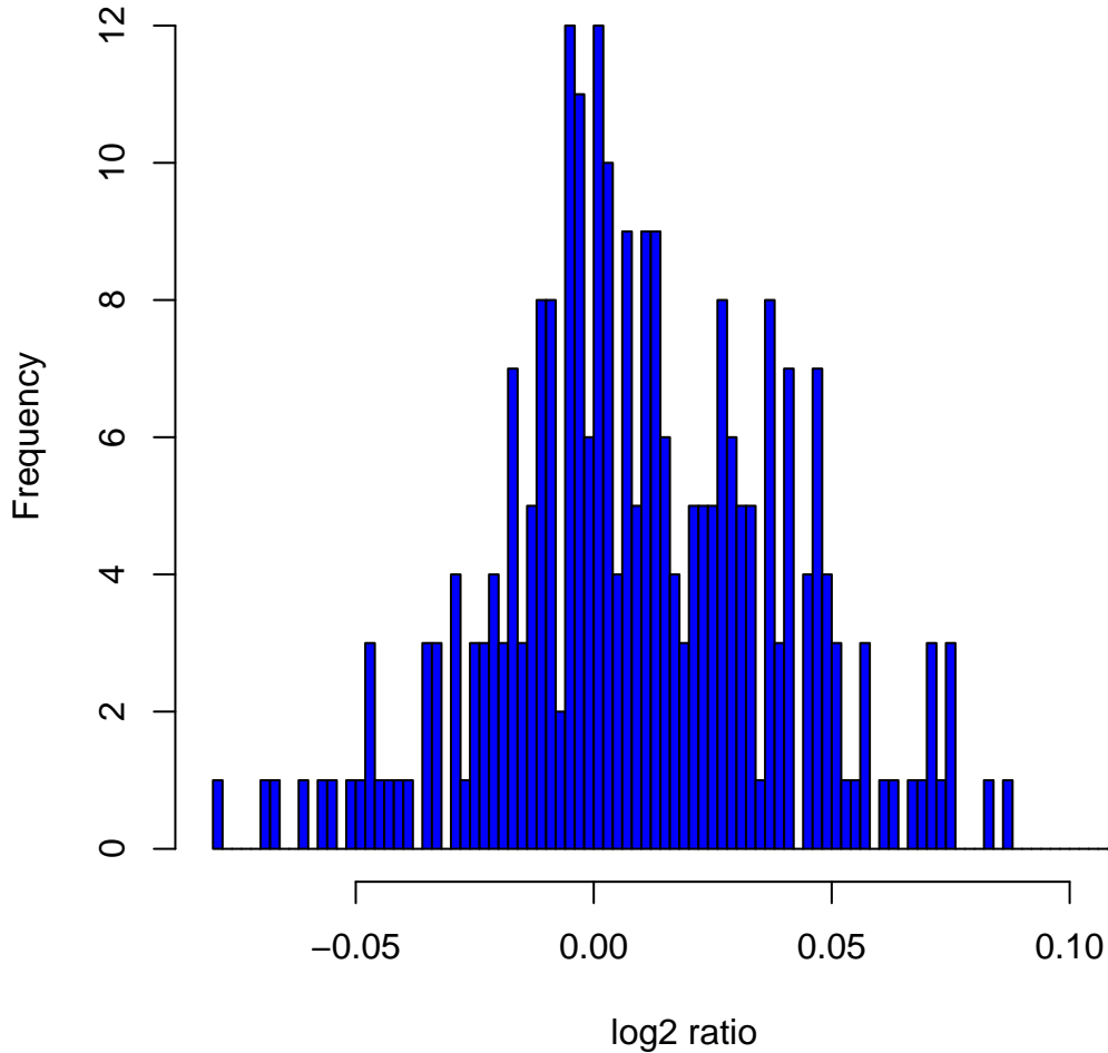
Histogram of log2ratios in 270 HapMap samples at clone Chr4tp-8F4
