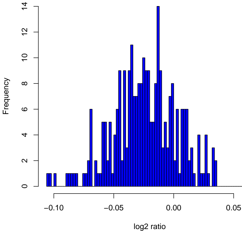
Histogram of log 2 ratios in 270 HapMap samples at clone Chr4tp-9B5
