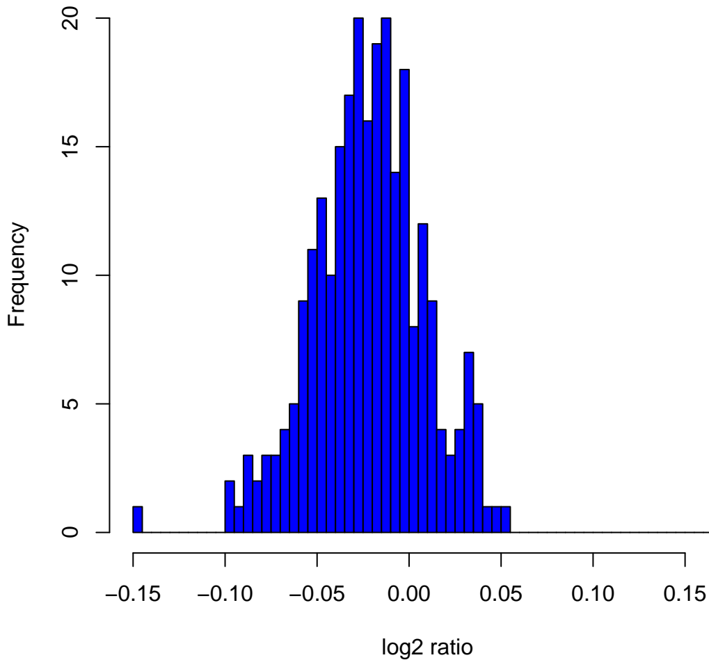
Histogram of log 2 ratios in 270 HapMap samples at clone Chr4tp-9B8
